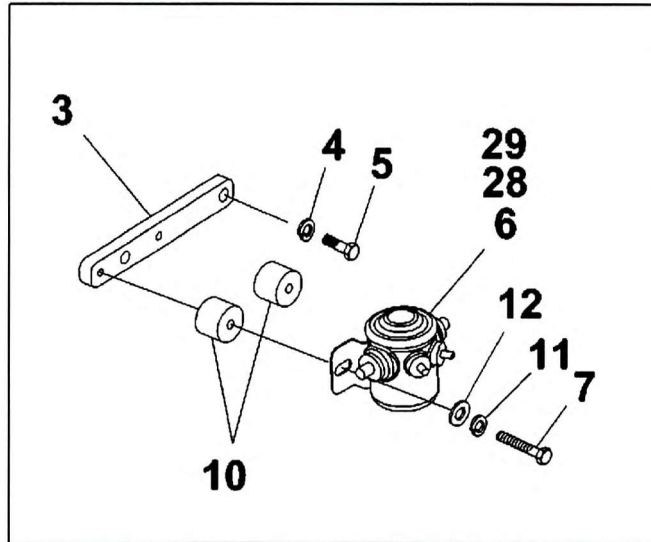
GRID HEATER SOLENOID RELAY
